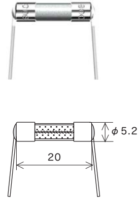
Lead wire diameter ϕ 0.8 (1 A–6.3 A) ϕ 1.0 (8 A–10 A) Scale: 1/1 (mm)
